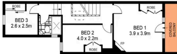
LEVEL ONE
