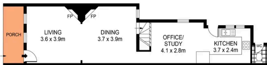
GROUND FLOOR
