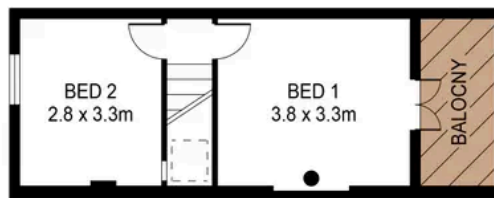
LEVEL ONE
