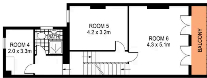
MID LEVEL
