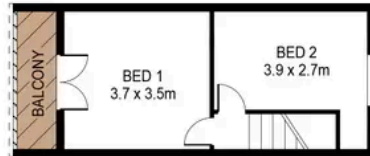
FIRST FLOOR
