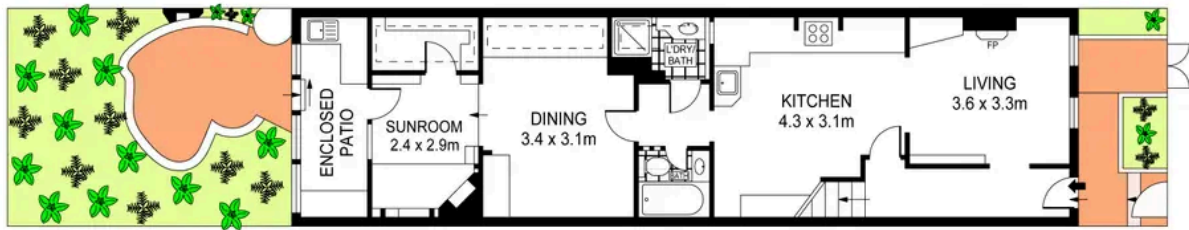
GROUND LEVEL
