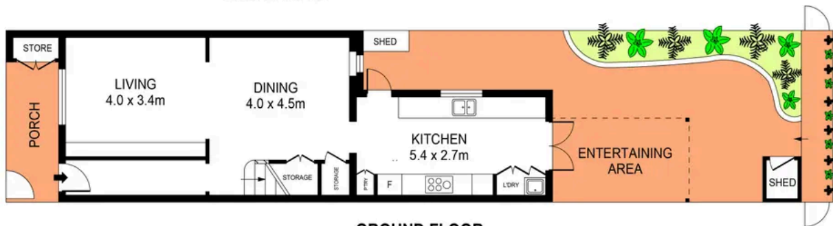
GROUND FLOOR
