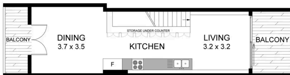
FIRST FLOOR
