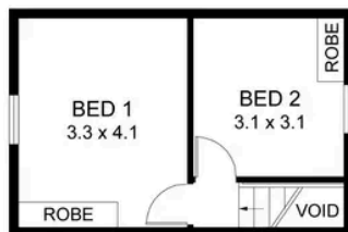
UPPER FLOOR
