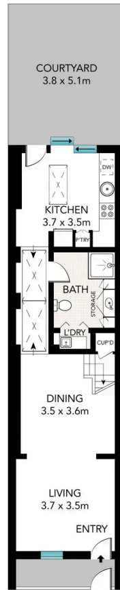
GROUND LEVEL
