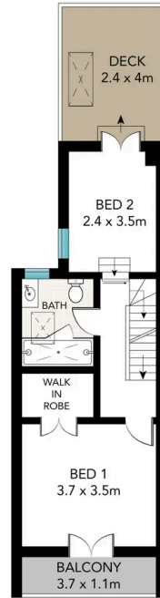
LEVEL ONE
