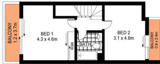
SECOND FLOOR
