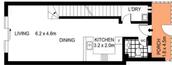
GROUND FLOOR
