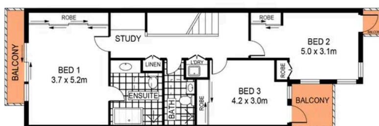
LEVEL ONE
