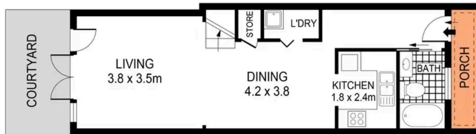
GROUND FLOOR
