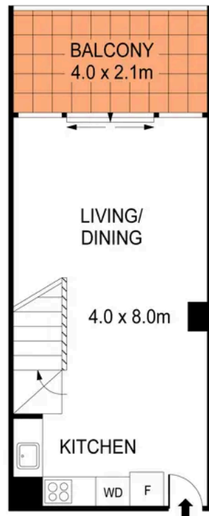
LEVEL TWO
