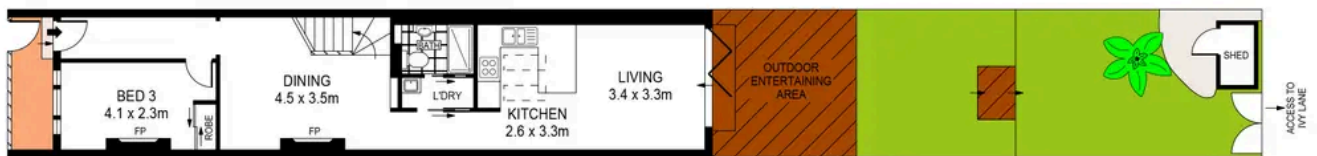
GROUND LEVEL
