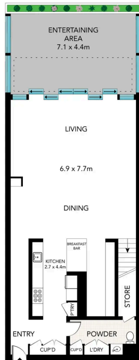
LOWER LEVEL
