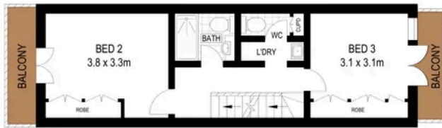
FIRST FLOOR
