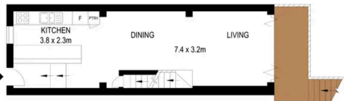
GROUND FLOOR
