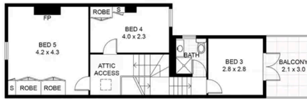
SECOND FLOOR
