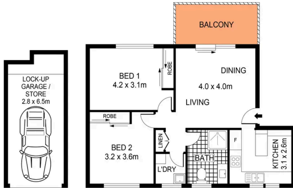
FIRST LEVEL
