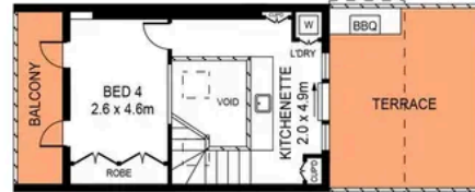
TOP FLOOR
