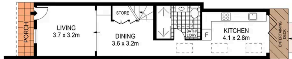
GROUND FLOOR
