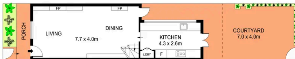
GROUND FLOOR
