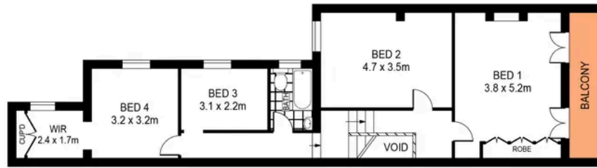
FIRST FLOOR
