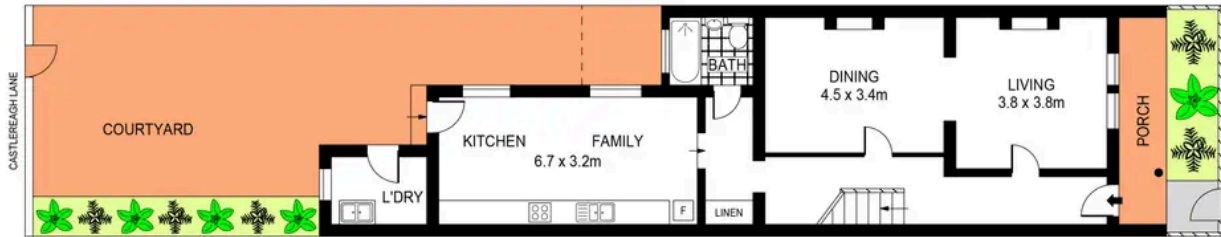
GROUND FLOOR
