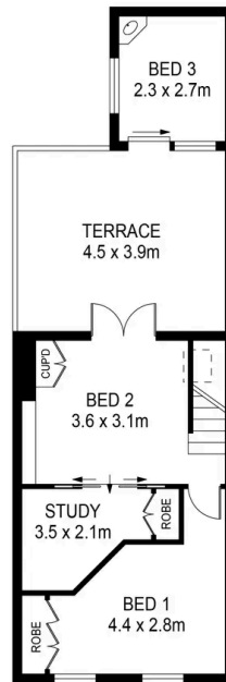
FIRST FLOOR
