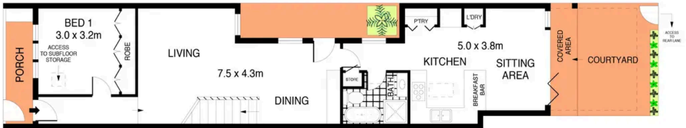
GROUND FLOOR
