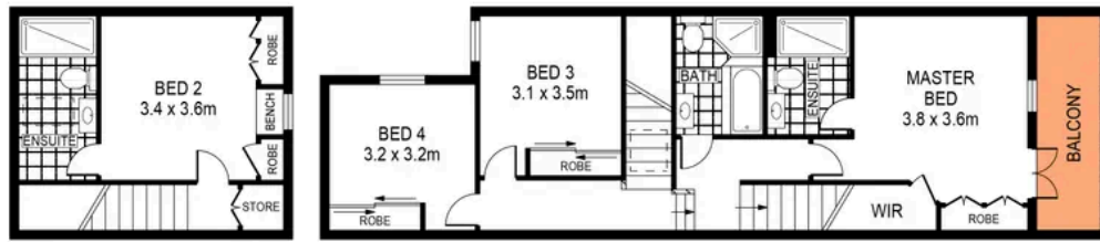
UPPER FLOOR
