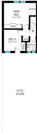
FIRST FLOOR
