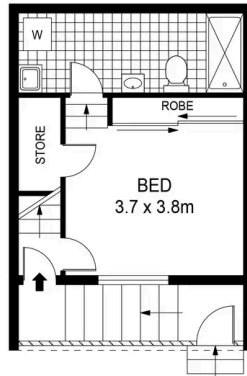
ENTRANCE LEVEL
