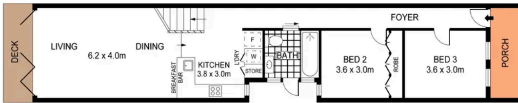
GROUND FLOOR
