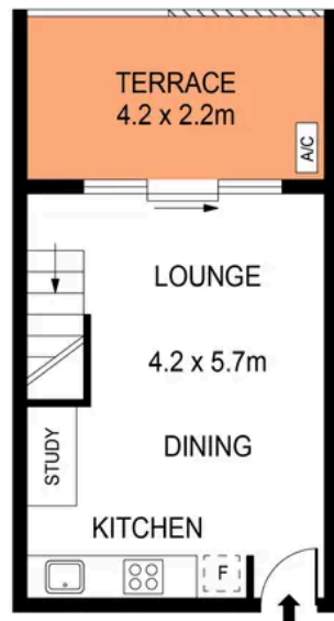
LOWER FLOOR
