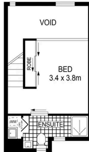
UPPER FLOOR
