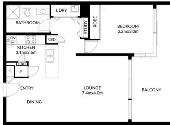
FLOOR PLAN
