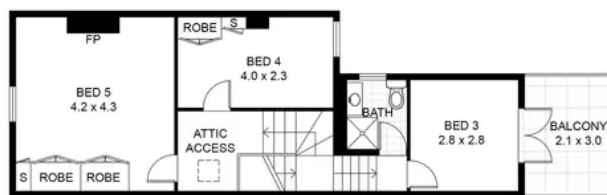
SECOND FLOOR
