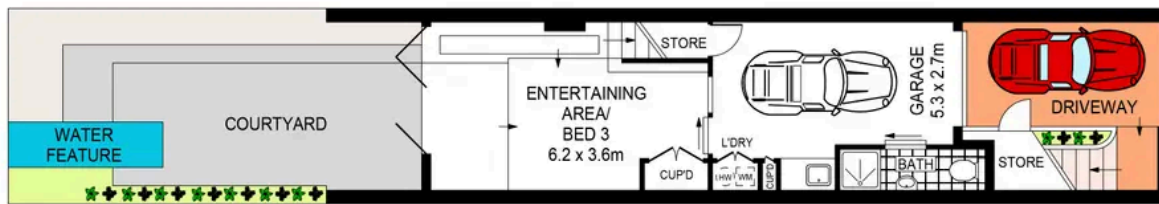
GROUND FLOOR
