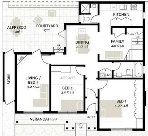
LEVEL 1
